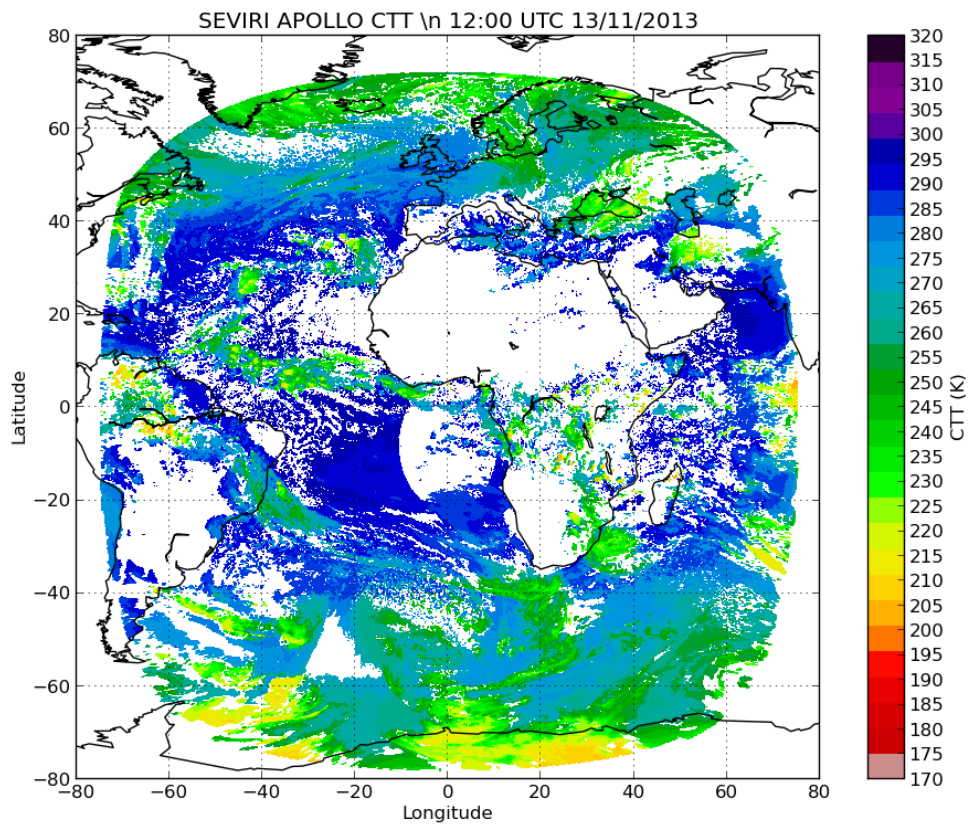
Fig. 12.5: Seviri Cloud top temperature
