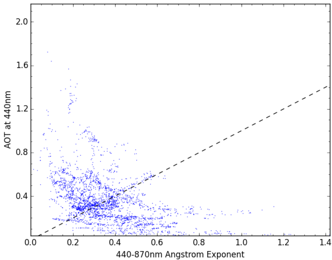
Fig. 12.7: Aeronet comparative scatter
