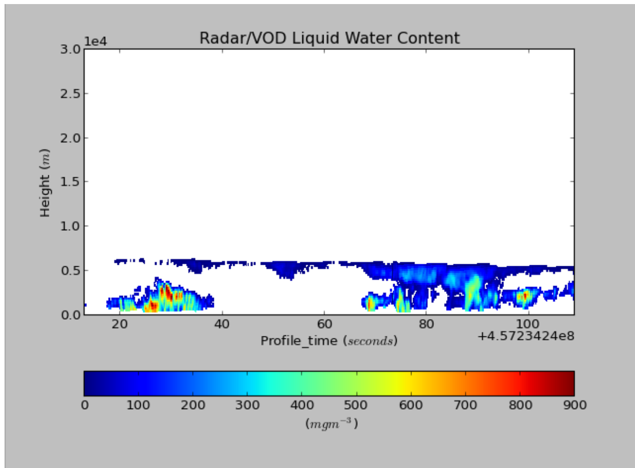
Fig. 12.11: CloudSat Liquid water content
