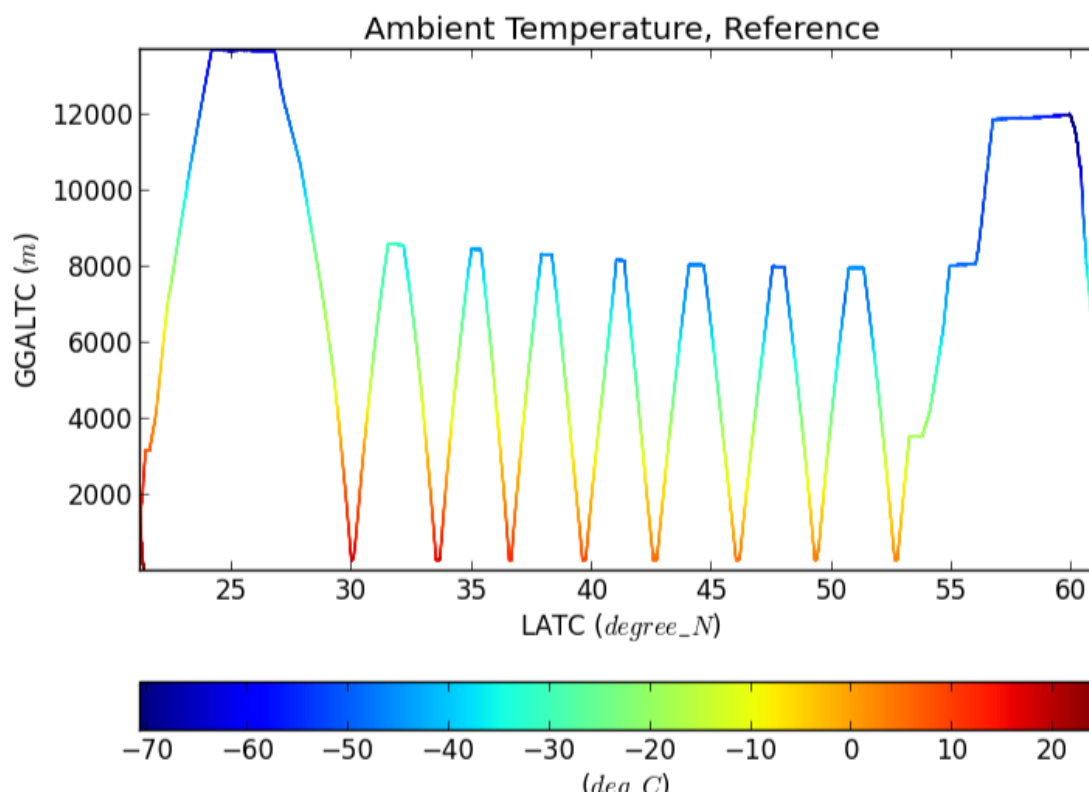
Fig. 12.13: NCAR-RAF ambient temperature
